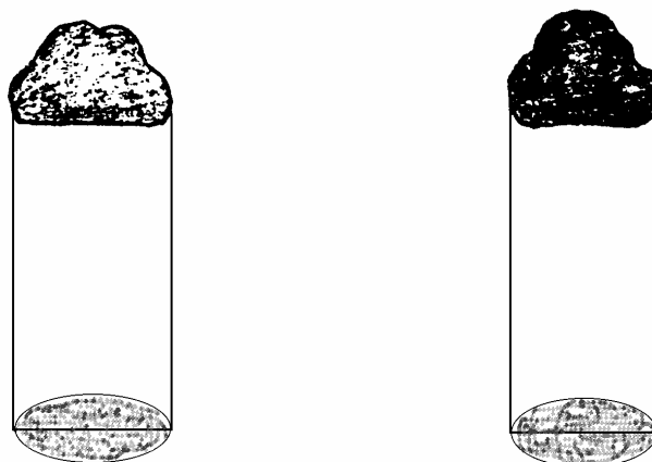
FIGURE 4 C Looking into or downwind and into or downsun.
