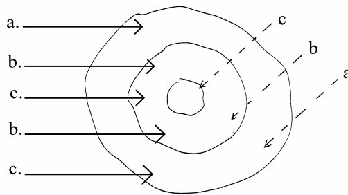
FIG 2. VERTICAL CIRCULATION IN A TYPICAL THERMAL.
