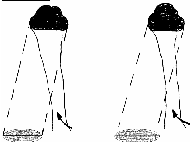
FIGURE 5 C Looking Downwind
