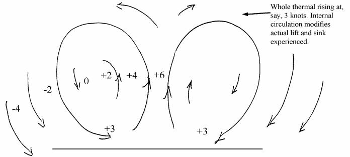
FIG 1 'CONTOURS' SHOW REGIONS OF SINK & LIFT.
