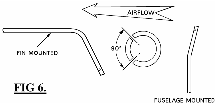
Fig 6. Irving Total Energy Tube
