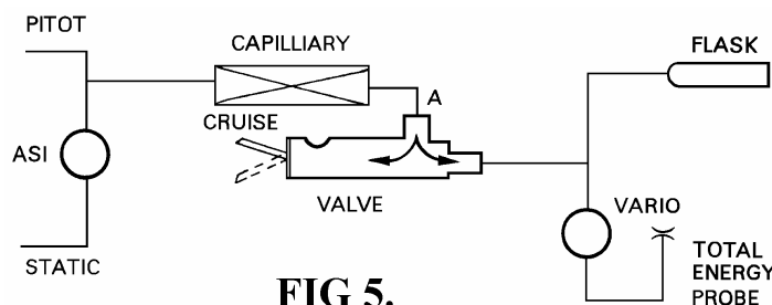
Fig 5. Netto Installation Layout
