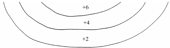
FIG 1 'CONTOURS' SHOW REGIONS OF SINK & LIFT.
