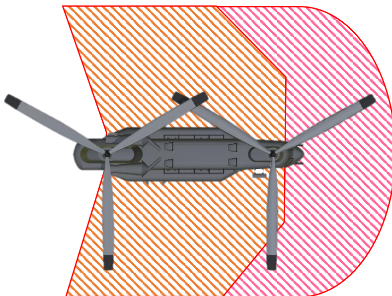
Figure 1: Guide to CH47 Chaff/Flare and rotor Danger Zones ◀
